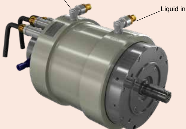
Liquid out
